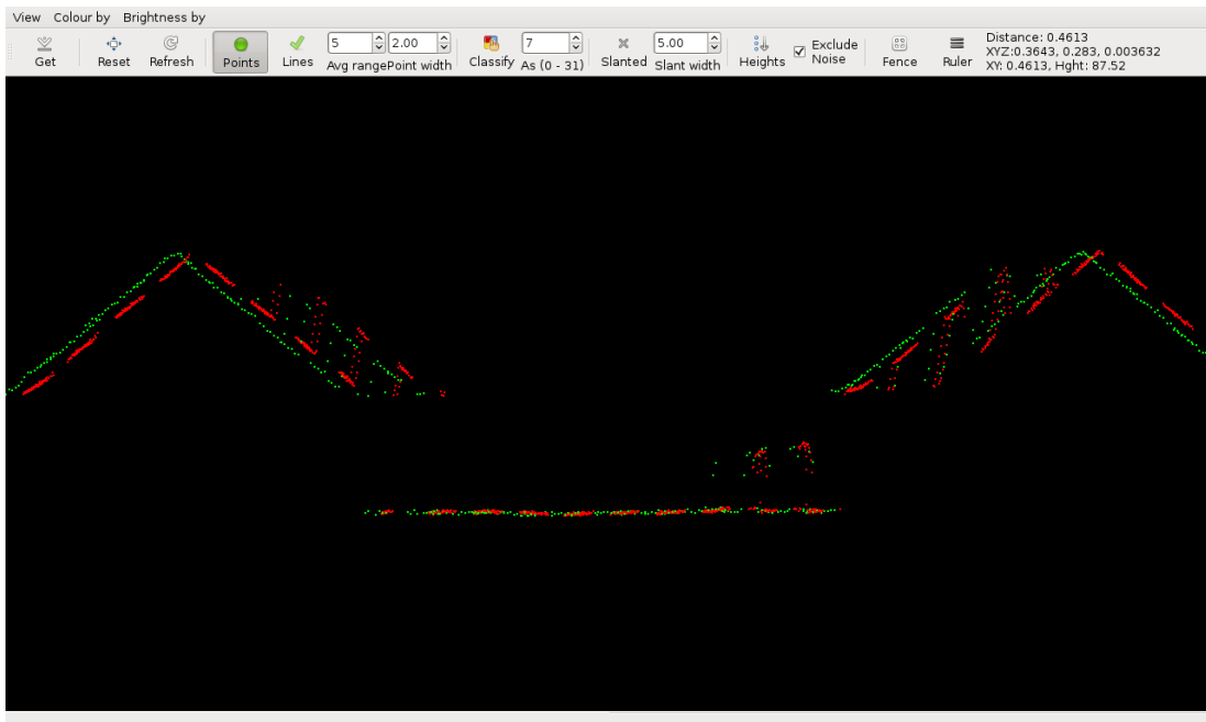
Figure 2: Horizontal difference is demonstrated most dramatically in the cross sections of rooftops along the length of two opposing flightlines. Points in the right-most projection are collected from a flightline headed south-west, while points in the left-most projection are from a directly opposite, north-east bound, flightline.
